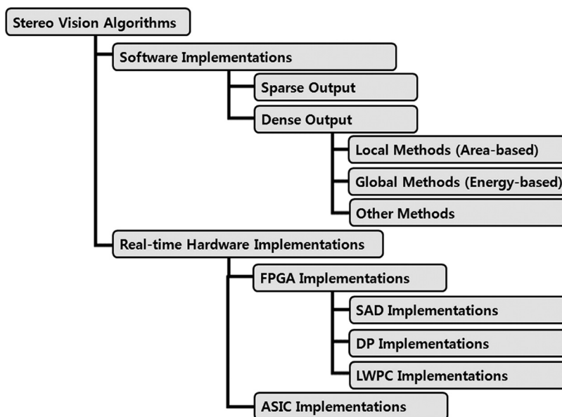
Figure 3. Categorization of stereo vision algorithms.
